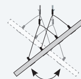
Suspension option 4:2 Tiltable in one axis (Front view/Sideview)
